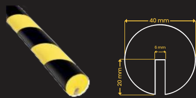
PROFILE PROTECTOR "A"
