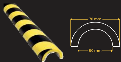
PIPE PROFILE PROTECTOR "O"
