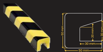
PROFILE PROTECTOR "V"
