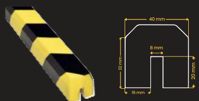
PROFILE PROTECTOR "U"
