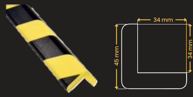
CORNER GUARD "L2"
