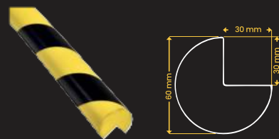
CORNER GUARD "C2"
