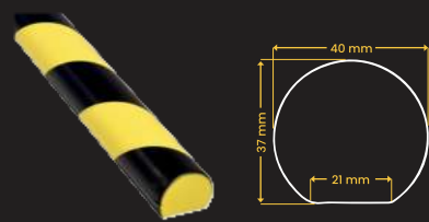
WALL PANEL PROTECTOR "D"
