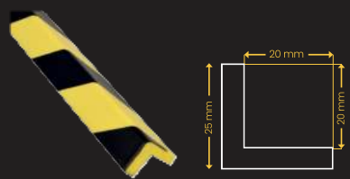
CORNER GUARD "L1"
