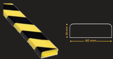
WALL PANEL PROTECTOR "I"
